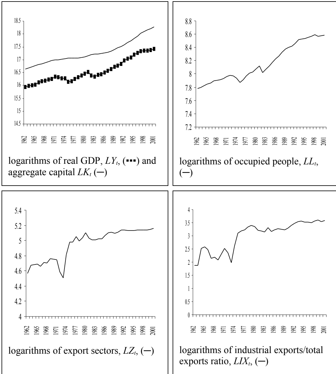
Figure 2: Time series used
